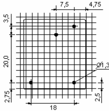
View of the soldering side. All measure in mm.
