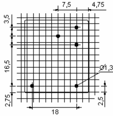
View of the solder side. All measure in mm.
